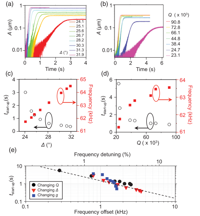
FIG. 4. Control of the oscillation start-up. (a) Envelope of the amplitude during start-up, for different \Delta 's, with Q = 120000 . The envelope is obtained through averaging multiple cycles of the oscillation around given times. (b) Envelope of the amplitude during start-up, for different Q 's, with \Delta = 27^\circ . (c),(d) Corresponding start-up time t_{\text{start-up}} and steady-state frequency extracted from (a) and (b), respectively. (e) The start-up time t_{\text{start-up}} versus the steady-state frequency offset, collected with different start-up conditions. The dashed line is a guide for the eye with a slope of -1 .
