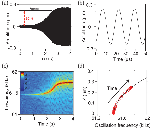
FIG. 3. Transient response during start-up. (a) Measured amplitude during oscillation buildup. The steady-state oscillation frequency is 61.7 kHz, with \Delta = 24.1^\circ . (b) Zoomed-in view of the steady-state oscillation of (a). The x axis is shifted arbitrarily. (c) Temporal frequency response of the oscillation. The power spectrum at each nominal time t_i is obtained by performing a nonoverlapping fast Fourier transform of the time domain data in a narrow window around t_i . (d) The temporal evolution of the oscillator on the amplitude-frequency plane, and a fitting to Eq. (3) (the black solid line). The extracted \beta is 1.05 \times 10^{11} \text{ m}^{-2} . The dc bias is 7 V for all of the data shown.
