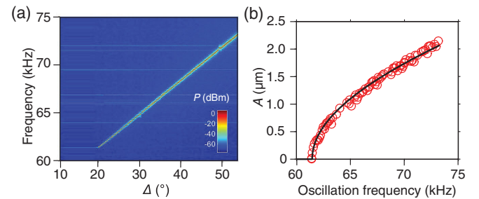
FIG. 2. Steady-state response of a nonlinear oscillator. (a) Measured power spectrum of the oscillation with different feedback-phase delay \Delta . Measurement at each \Delta is performed with a time constant long enough to ensure that the transient response has died out. The dc bias is 7 V. (b) Extracted steady-state oscillation amplitude and frequency (the red circles), and a fitting to Eq. (3), with \beta = 1.15 \times 10^{11} \text{ m}^{-2} .
